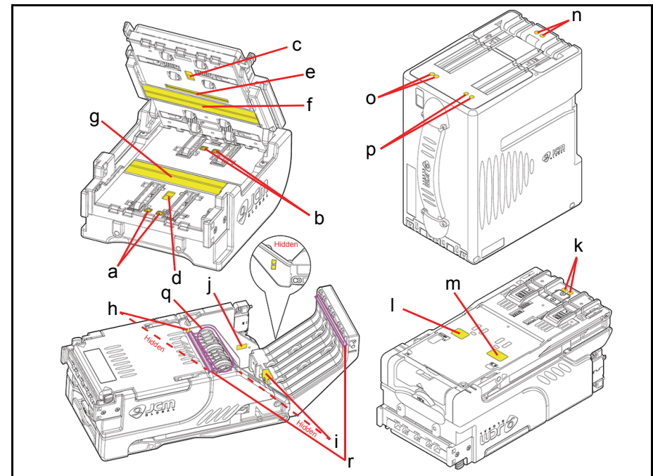
Figure 10 iVIZION Sensor Locations
