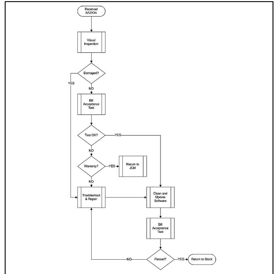
Figure 3 iVIZION Repair Process Flowchart
