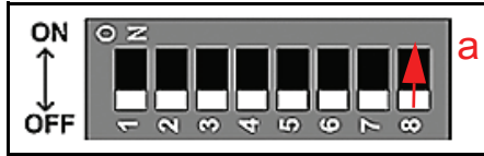
Figure 6 DIP Switch SW1
